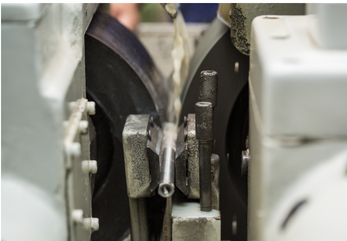
Centerless grinding process
