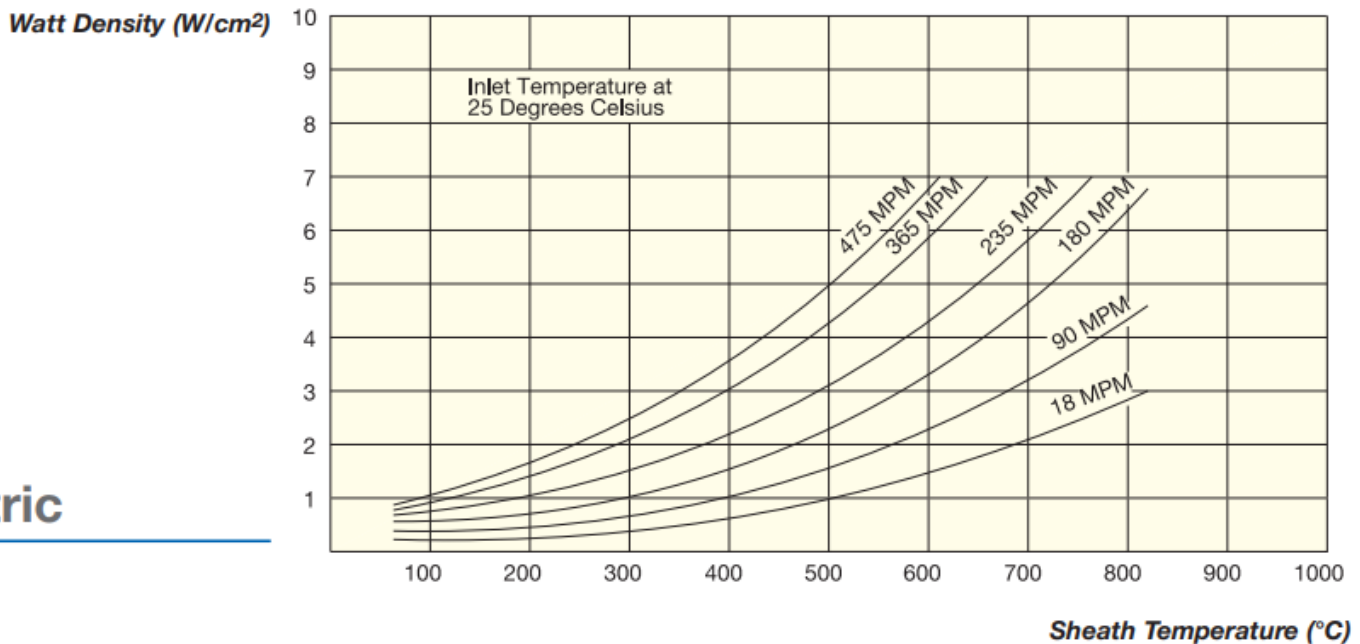
Fig 3. Watt Density vs. Sheath Temperature
